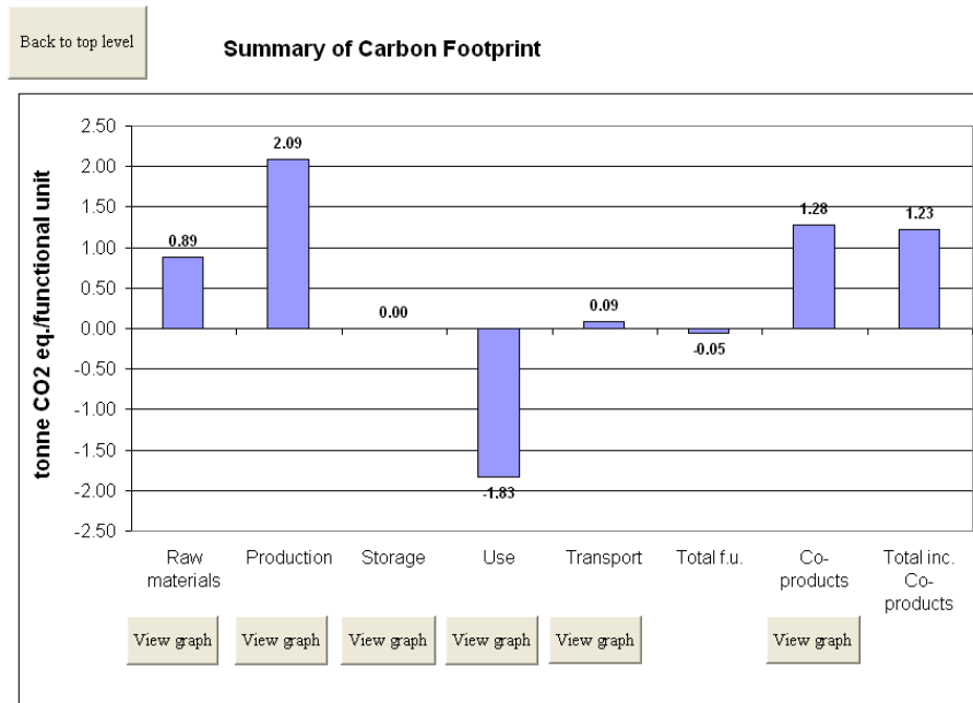
Figure 24 Graphical view of carbon footprint results at the top level of the tool
